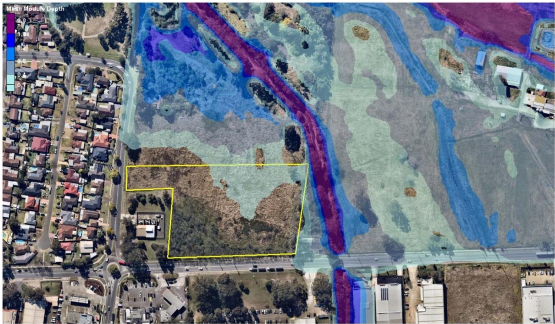
Figure 9 – Existing Flood Mapping
