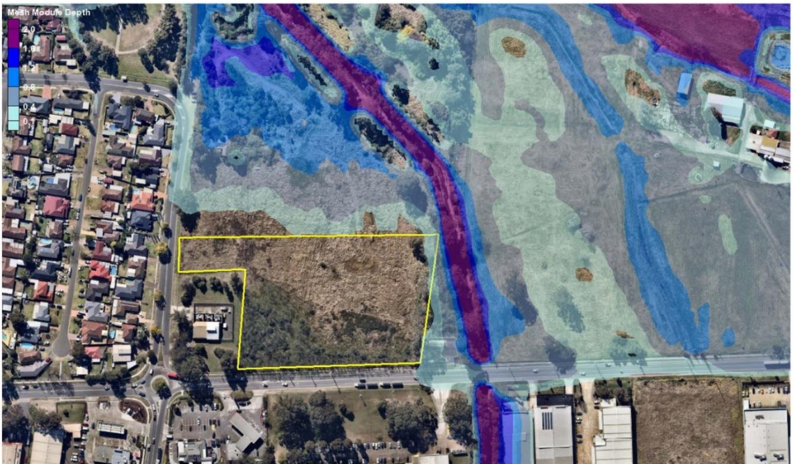
Figure 10 – Post Development Flood Mapping
